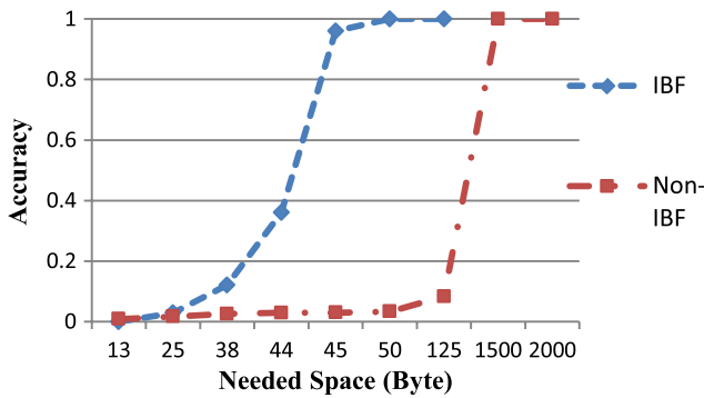
Fig. 30. The IBF versus Relational structure in terms of needed space.
