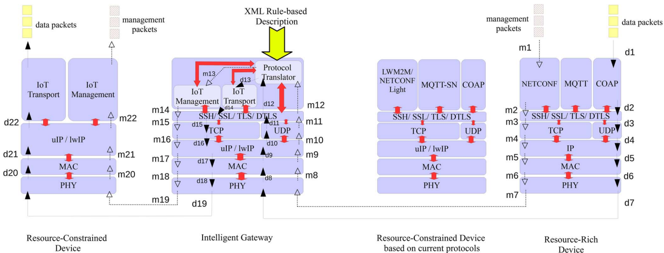
Fig. 26. The Architecture of a rule-base Intelligent IoT gateway.
