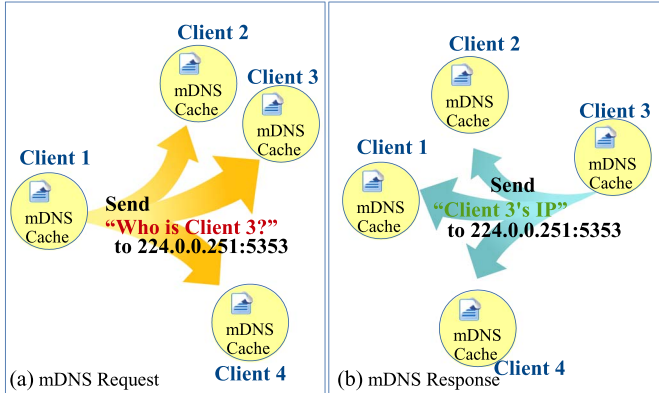
Fig. 17. Request/Response in mDNS protocol.
