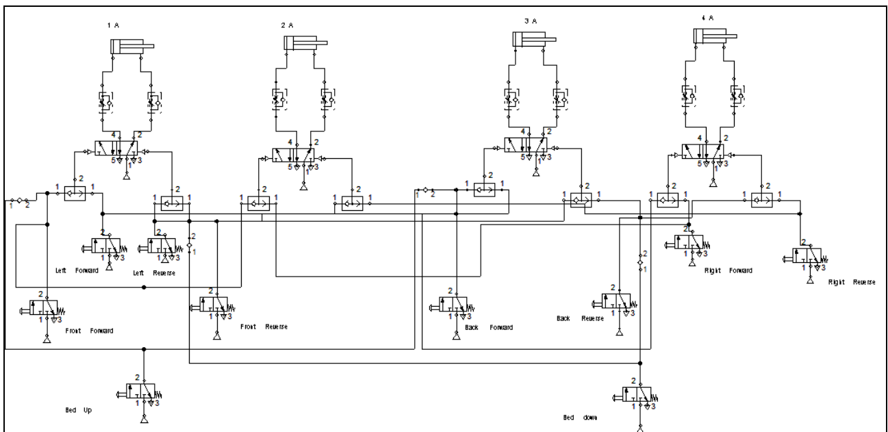
Figure 3. Pneumatic circuit in bed stable position
