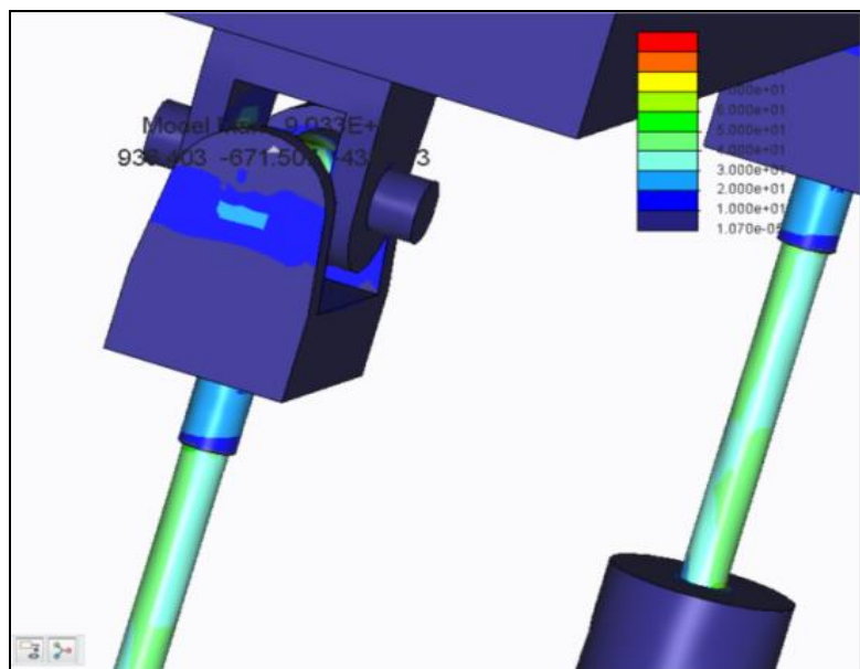
Figure 11. Maximum stress
