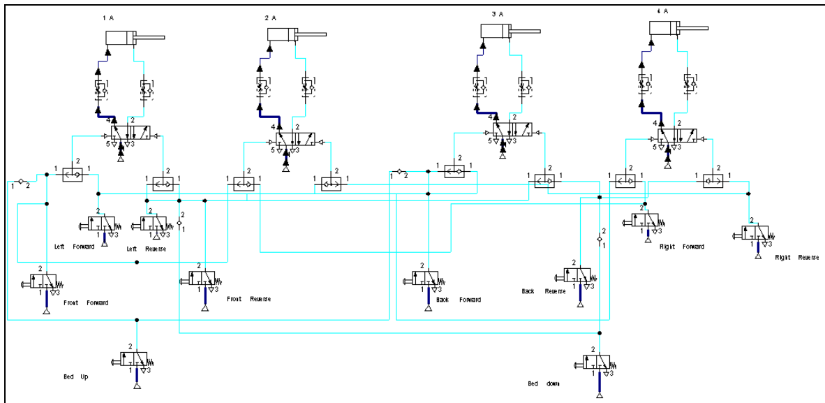
Figure 7. Left side inclination
