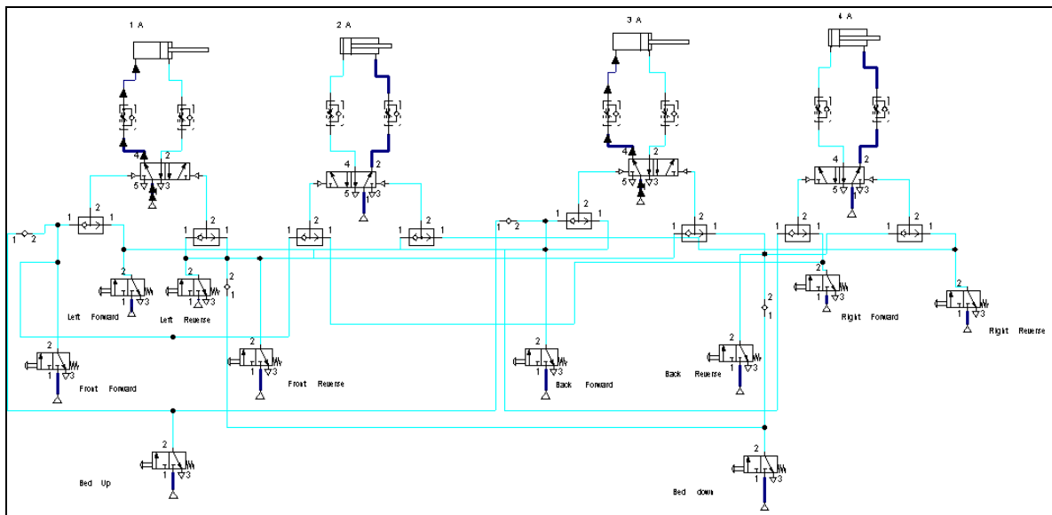
Figure 8. Pneumatic design for raise of bed
