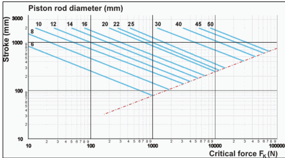
Figure 12. Stroke length, piston rod diameter and critical force relation diagram (Courtesy: Engineering Tool Box)
