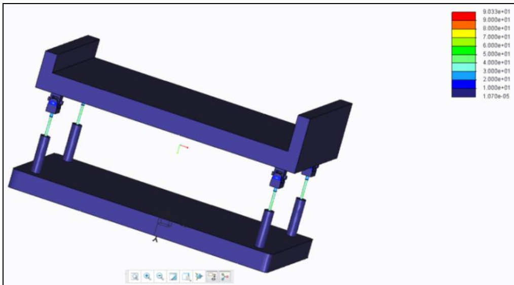
Figure 10. Von-Mises stress analysis
